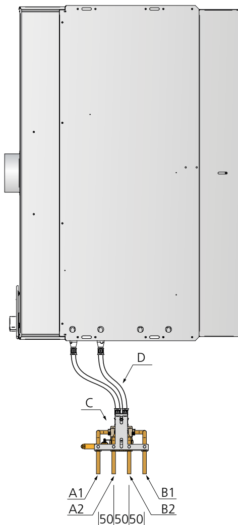
Figure 23. Water connection, CCO valve.
