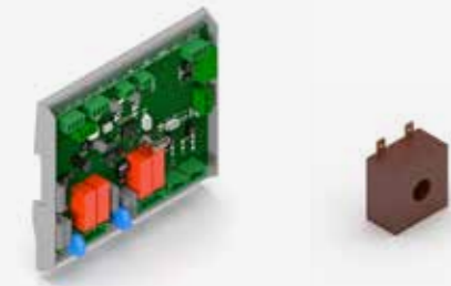
EHHKX expansion control required when two hydraulic steam production units are used
