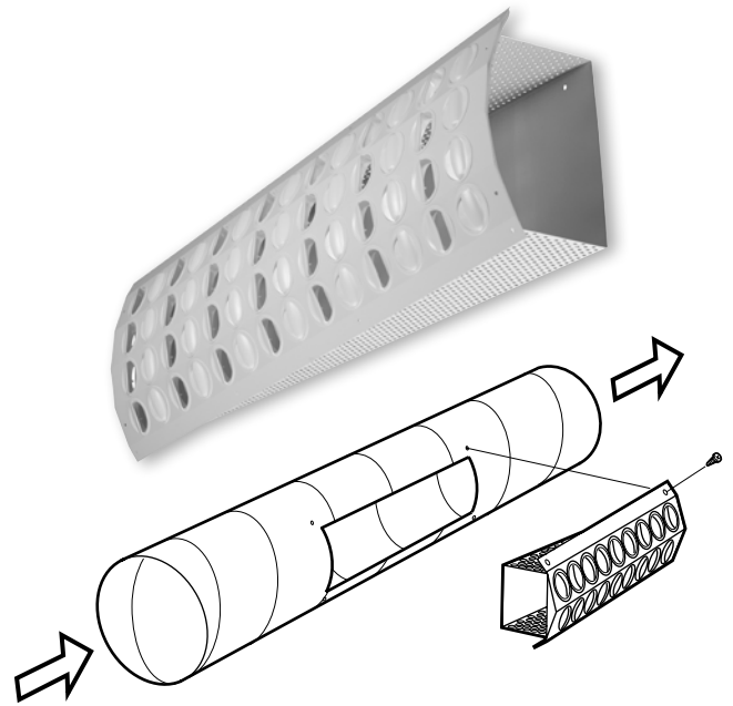
Figure 1. Installation.
