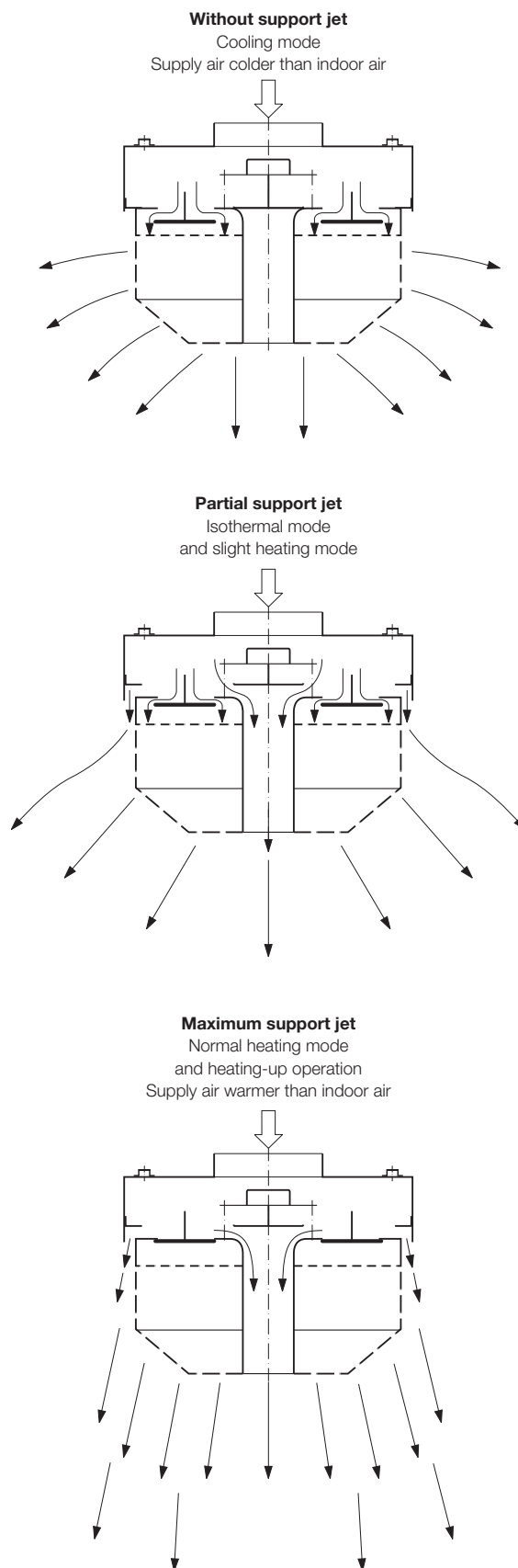
Fig. 3: Sketch of discharge pattern
