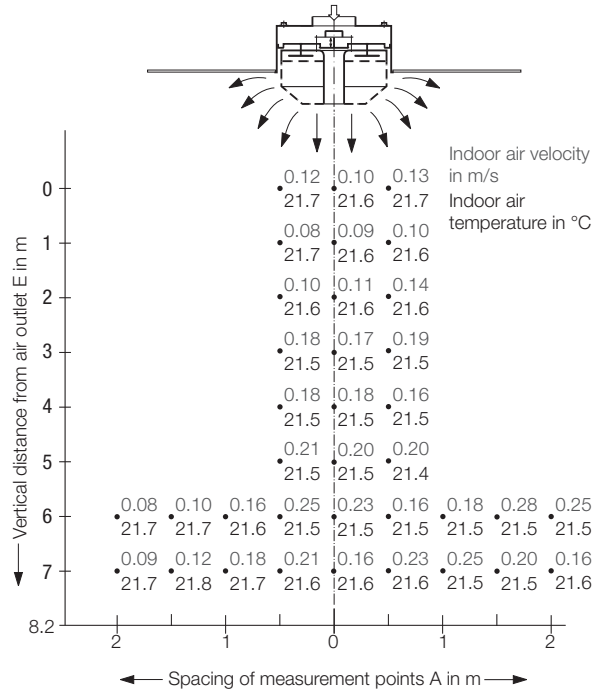
Fig. 7: Indoor air velocities and temperatures with air outlet volume flow rate of 695 l/s [2 500 m³/h] and \Delta\vartheta_K = -5 K (cooling mode)
